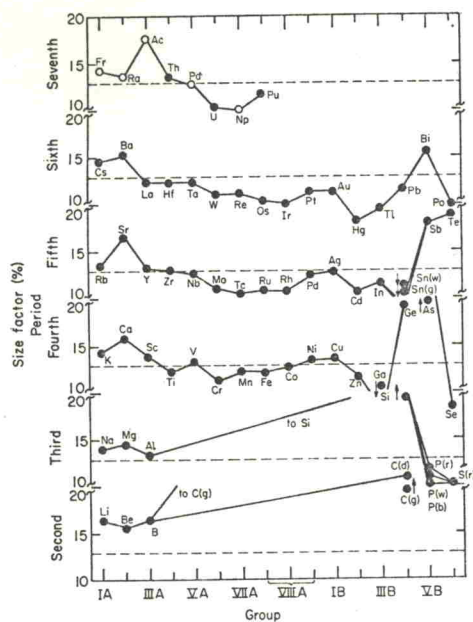
FIG. 34. Size factor (final best representative value) of all of the elements considered in this review with the exception of the rare-earth metals. The horizontal dashed line represents the mean value. Open points are estimated data.
